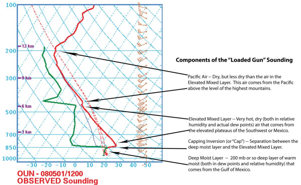
Figure 2: Skew-T Log-p Sounding for KOUN 12 UTC 1 May 2008. This sounding illustrates the so-called "Loaded Gun" Sounding, often associated with the development of severe thunderstorms.
