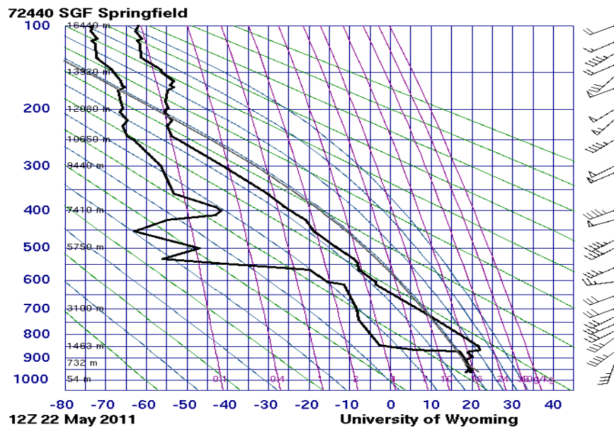
Figure 1: KSGS Sounding, 12 UTC 22 May 2011
